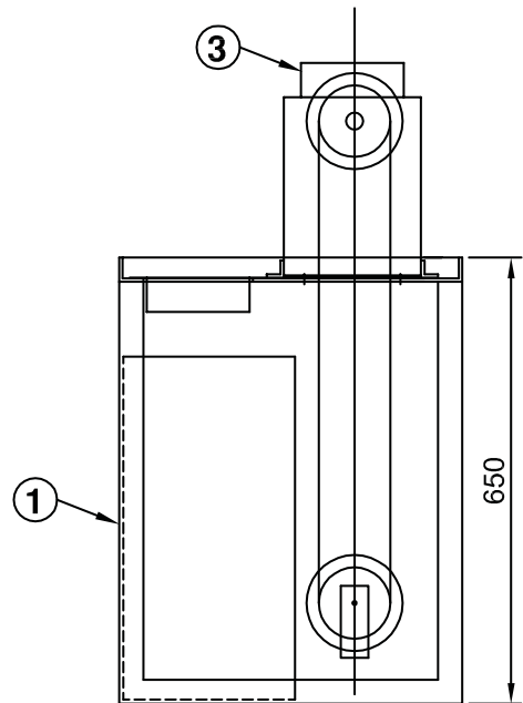
GA FOR OIL SKIMMER & STAND FOR 15 LPH
